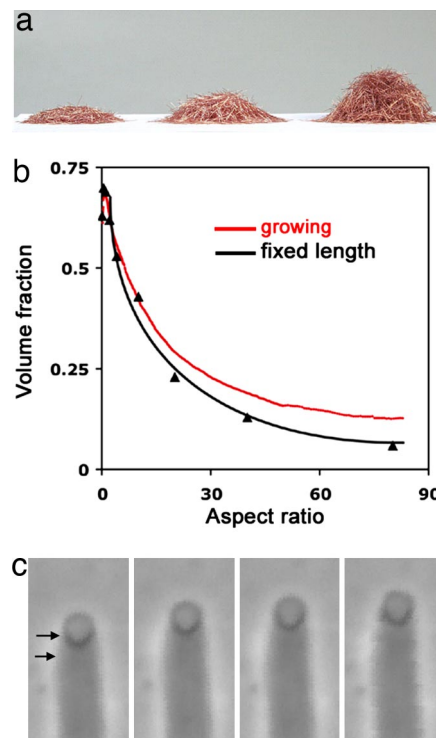
Fig. 2. Packing of rigid rods. (a) Illustration of how rod length influences packing density. Each pile of rods was formed from 15 g of chopped copper wire, prepared by sprinkling onto a flat surface. The rod lengths were 8, 12, and 16 mm, left to right. The rods in the piles do not stick to one another but, especially the high-aspect ratios, form relatively stiff solid-like entangled structures. The piles were all incompressible. Although the persistence length to contour length ratio of the wire shown here is greater than that of MSP filaments in fibers, similar effects are seen with semiflexible rods (18). (b) Simulations indicate that growing rods (red) pack similarly to rods of fixed length (black) and, for both, the volume fraction is approximately inversely proportional to the rod aspect ratio. (c) Phase-contrast images taken 5.5 sec apart of the vesicle-bearing end of a fiber growing at an average rate of 8 μm/min -1 . The lines indicate the region close to the vesicle where the diameter of the fiber expands, which also moves forward as the fiber grows. (Scale bar, 2 μm.)
